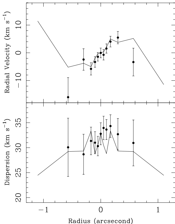
FIG. 1.— Radial velocity and velocity dispersion profile of G1 from the STIS observations. The points and the uncertainties come from the unsymmetrized measurements. The solid lines come from the symmetrized estimate that are used in the dynamical modeling. There is a single ground-based estimate of the dispersion that is not shown here; Djorgovski et al. (1997) measure \sigma = 25.1 \pm 1.7 km s ^{-1} in a 1''.2 \times 3''.0 aperture.
