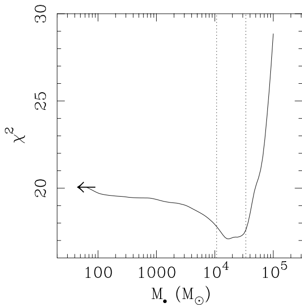
FIG. 3.— \chi^2 as a function of BH mass. We have marginalized over M/L . The vertical dashed lines denote the 68% confidence band quoted for the BH mass uncertainties. The arrow on the leftmost point indicates that this point is actually at zero BH mass, off the edge of the panel.
