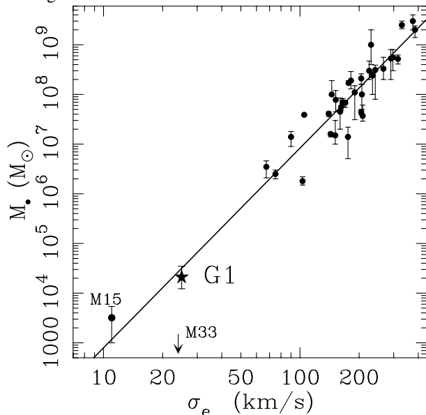
FIG. 4.— The M_\bullet - \sigma correlation for nearby galaxies, adapted from Tremaine et al. (2002). We include here the upper limit for M33 (Gebhardt et al. 2001), the BH mass estimate for the globular cluster M15 (van der Marel et al. 2002 and Gerssen et al. 2002), and the mass for G1. The solid line is the linear fit given by Tremaine et al., which does not include the cluster G1 or M15.
