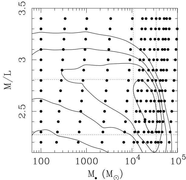
FIG. 2.— Two-dimensional plot of \chi^2 as a function of BH mass and M/L for G1. The points represent models that we actually ran. The contours were determined by a two-dimensional smoothing spline interpolated from these models, and represent \Delta\chi^2 of 1.0, 2.71, 4.0, and 6.63 (68%, 90%, 95%, 99% in projection). The vertical lines are the 68% limit for the BH mass, and the horizontal lines are the 68% limit for M/L .
